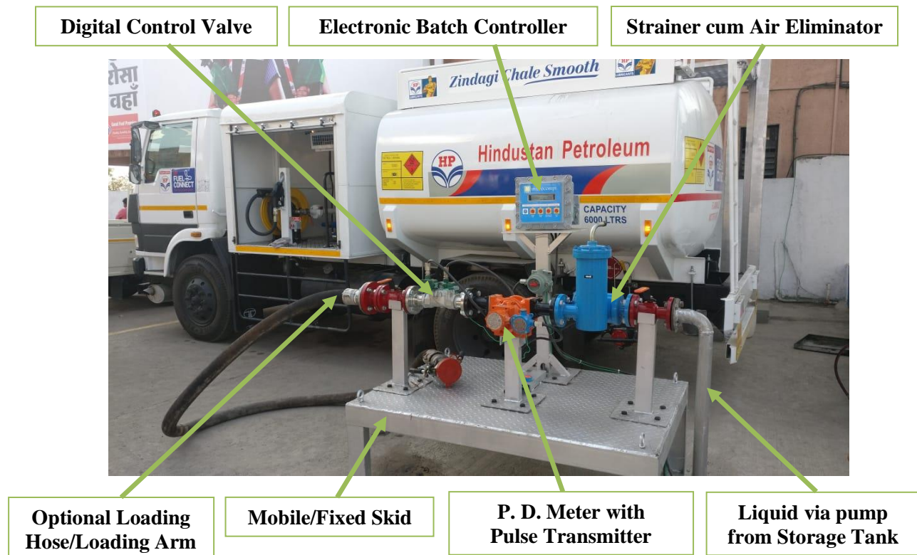
Pic. 1: P. D. Flowmeter in Bottom Loading operation at a location
