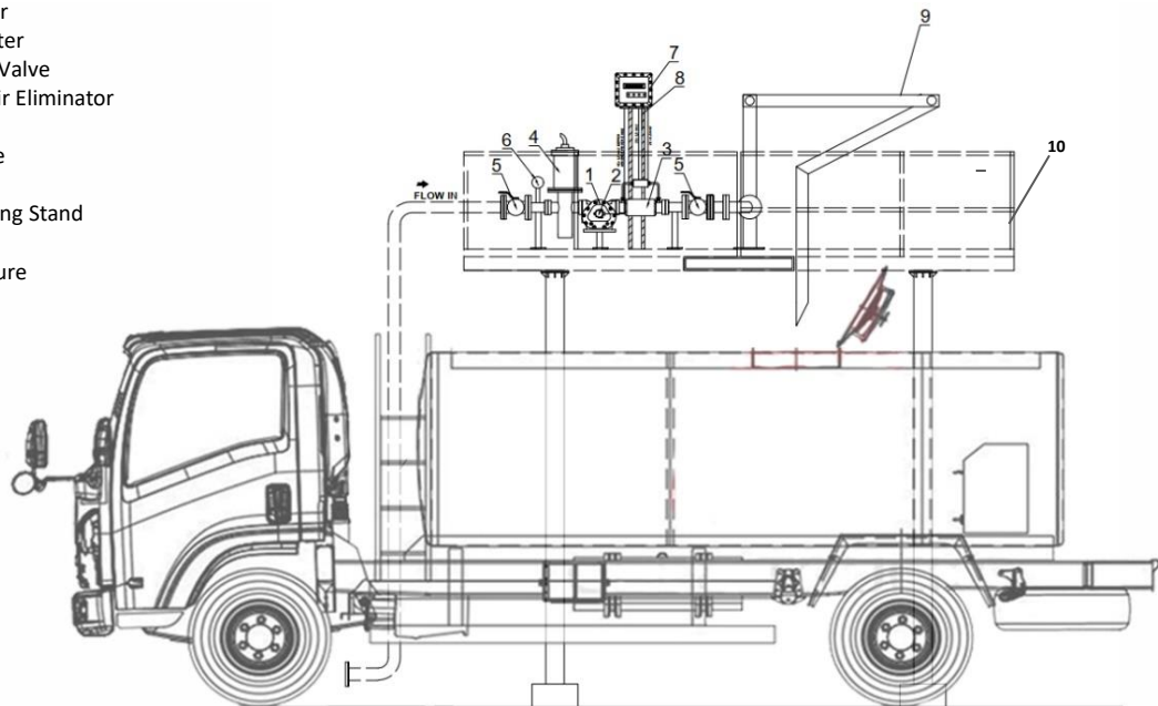
Pic. 2: Typical Top Loading Arrangement
